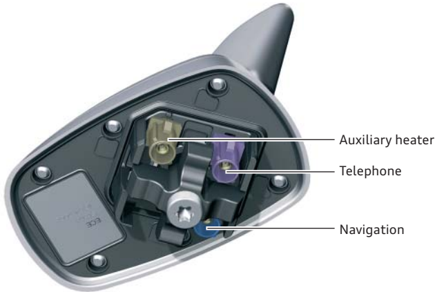
Roof aerial R216 (Europe/rest of world)
