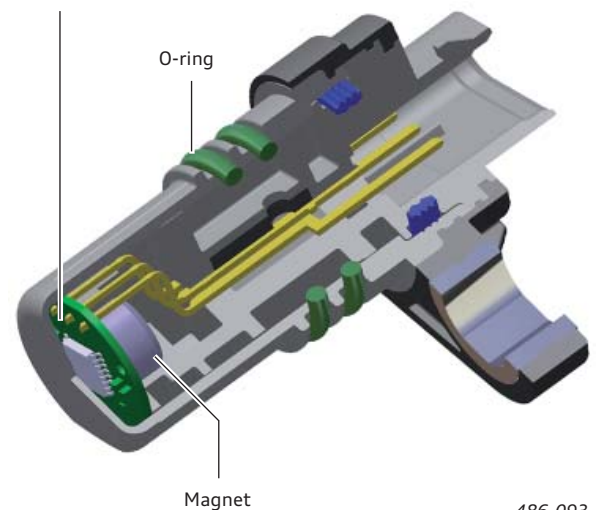
PCB with 4 Hall sensors
