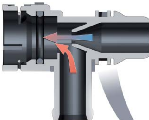
Return line from heater heat exchanger
