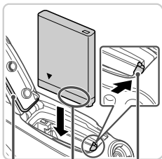
Terminals Waterproof Seal Battery Lock
