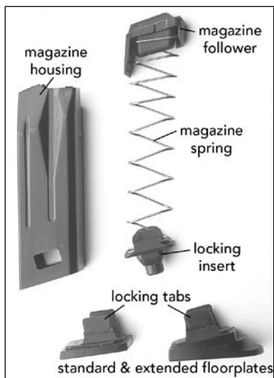
Figure 22 - 10 rd. magazine
