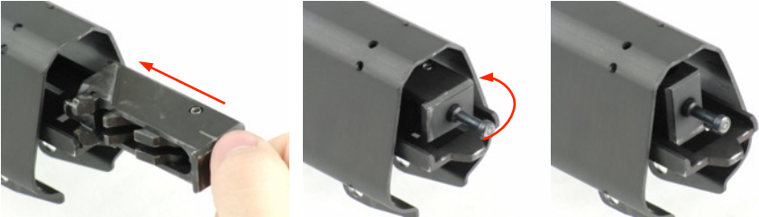
Figure E-5: Insert Bolt onto Bolt Carrier Sideways and Rotate 90°
