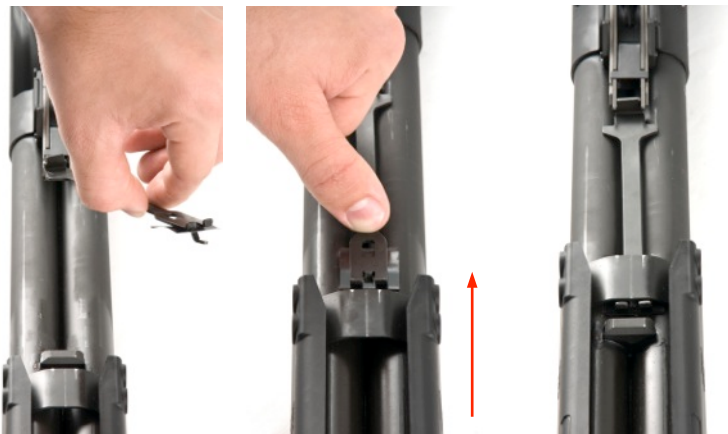
Figure E-3: Slide Forend over DFE Link Legs to Secure Assemblies
