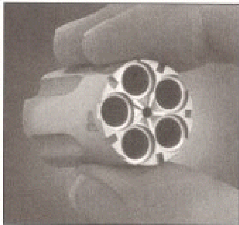
Hammer safety slots in between cartridge chambers
