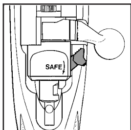
Figure 5. Safety selector in “ FIRE ” (full forward) position. The safety selector should be moved to this position only when the gun user is actually firing the rifle. When the safety is in the fire position, it is referred to as being “off.” (When the safety is in the “SAFE” position, it is referred to as being “on.”)
