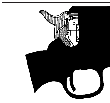
4. With trigger held fully rearward, the hammer actuates firing pin through transfer bar.
