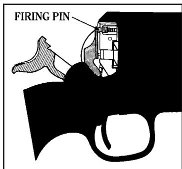
3. Hammer at full-cock. Top of the transfer bar is aligned with firing pin.
