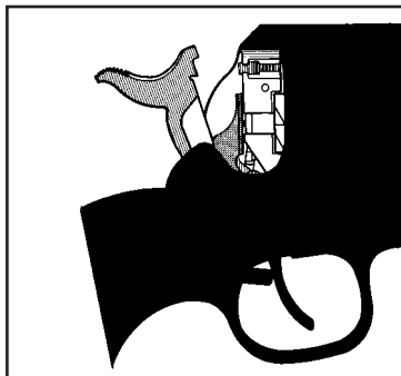
2. Hammer in loading notch position. For loading and unloading only . See "Safe Carrying Position Warning", p. 17.
