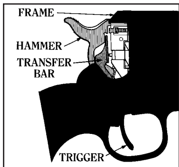
1. Hammer nose on frame. Trigger forward. Transfer bar is below firing pin. This is the "Safe Carrying Position" for Bearcats with serial numbers above 93-00000 only .
