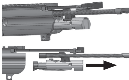
CARRIAGE ASSEMBLY
