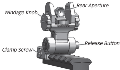
REAR SIGHT WINDAGE ADJUSTMENT
