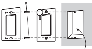
Existing Wall Box (No Anchor)
