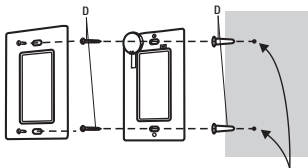
Drill 2 pilot holes & insert anchors
