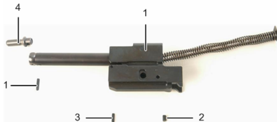
Figure 8-89. Bolt Carrier Assembly
