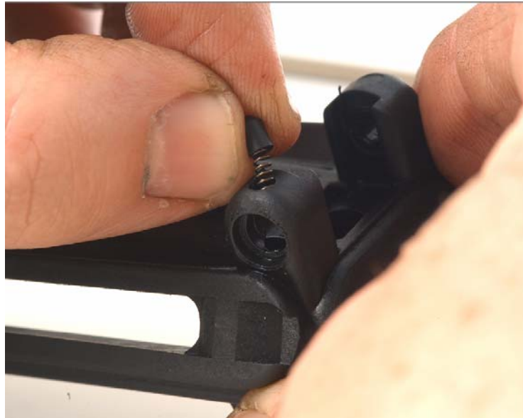
Figure 8-67. Inserting the Windage Screw Plunger
