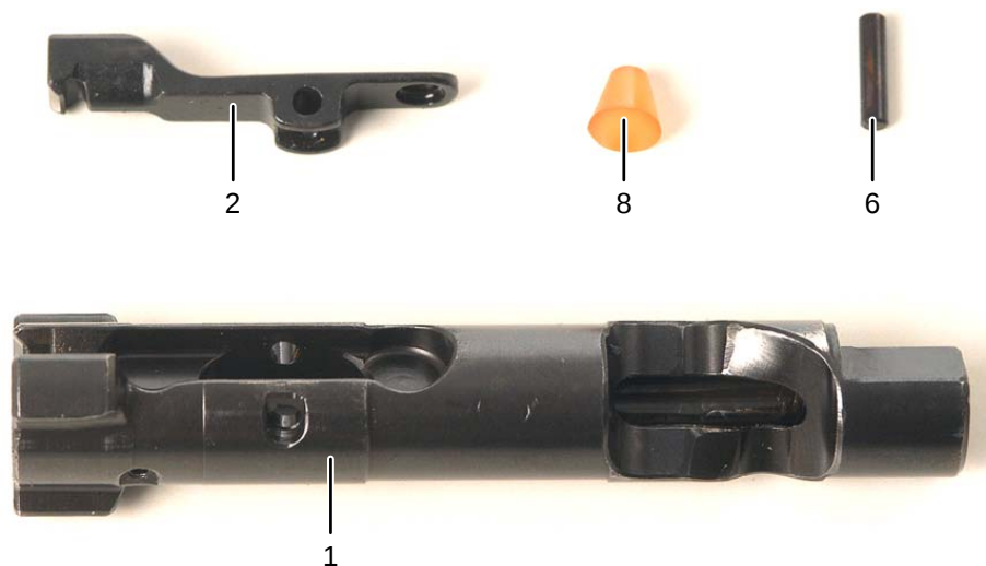
Figure 8-57. Bolt Assembly
