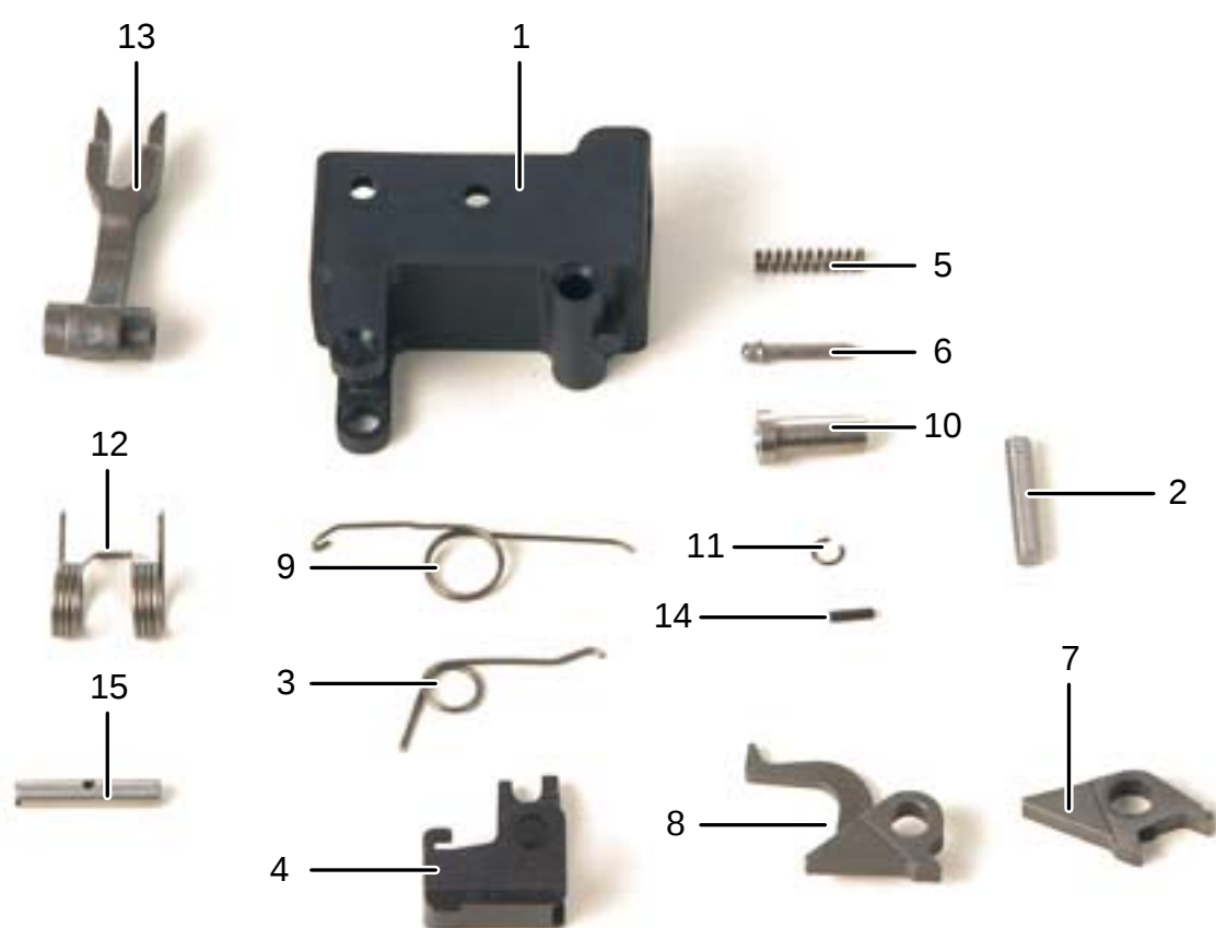
Figure 8-94. Mechanism Assembly
