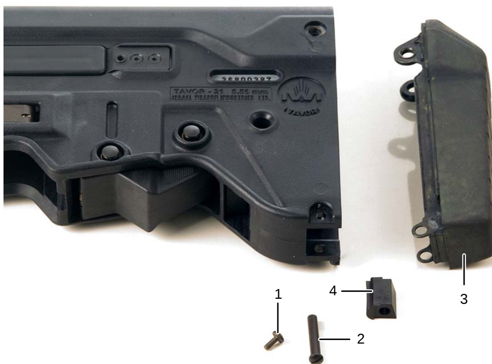
Figure 8-38. Butt Assembly
