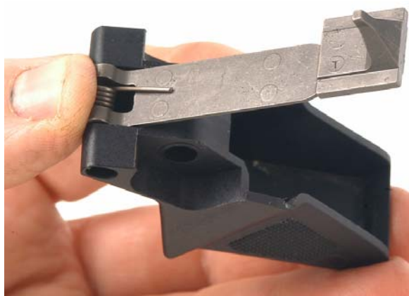
Figure 8-44. Installing Bolt Carrier Stopper
