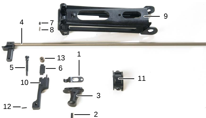
Figure 8-66. Cocking Handle Guide Assembly
